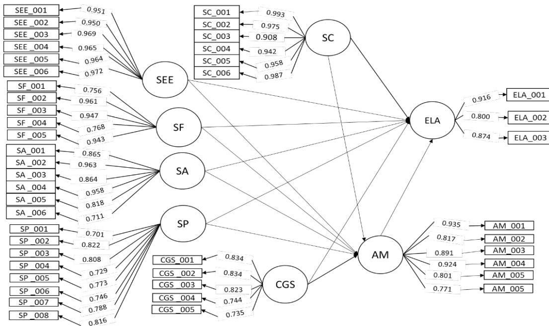
Figure 2. Algorithm Result
