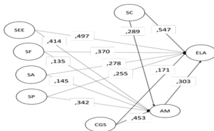
Figure 4. Path Coefficients
