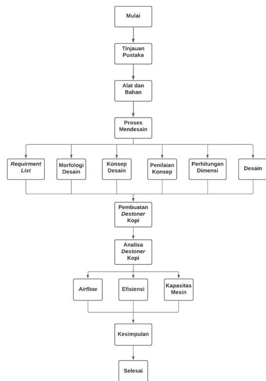
Gambar 1. Alur Penelitian
